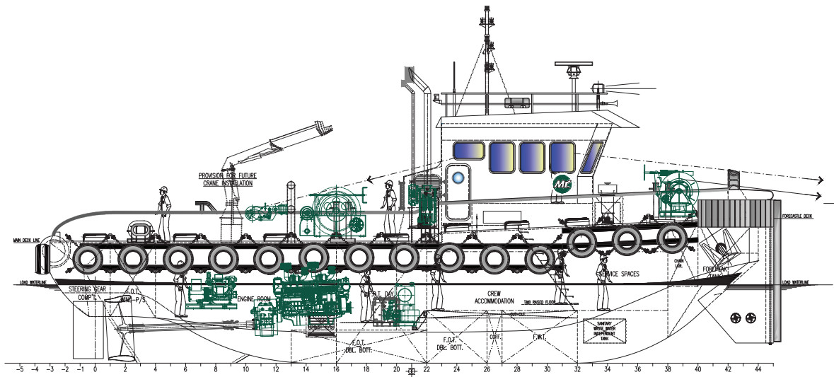
Outboard profile
