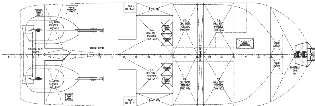
Tank plan
